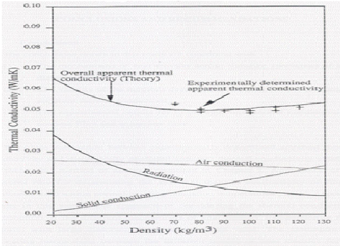
Figure 1. Apparent thermal conductivity of sugarcane fibre (Manohar, 1991).
