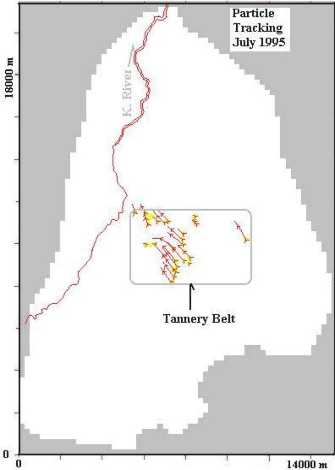
Figure 8. Groundwater streamlines computed for 7 years since 1988
