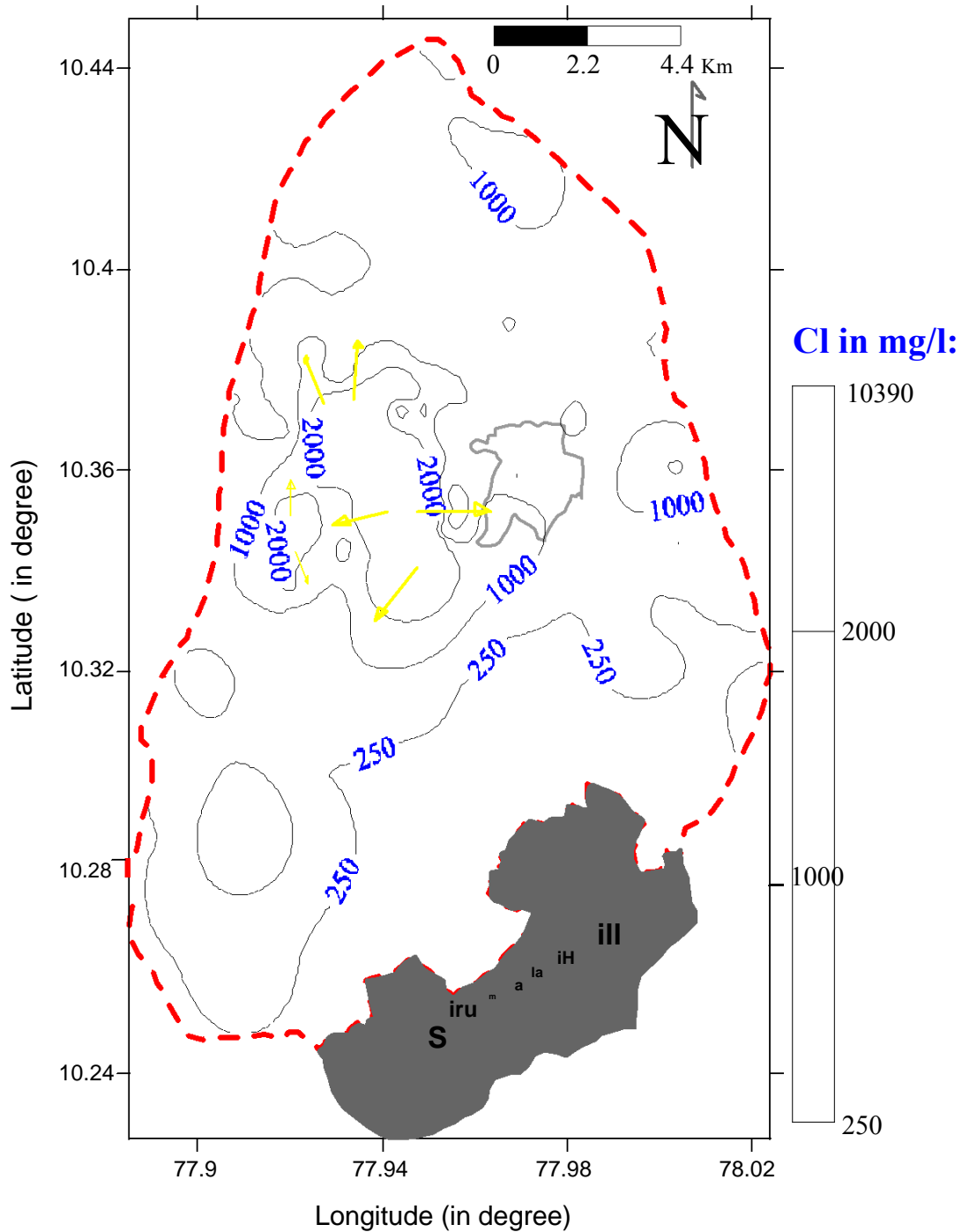
Figure 5. CI shaded map (January 2001)
