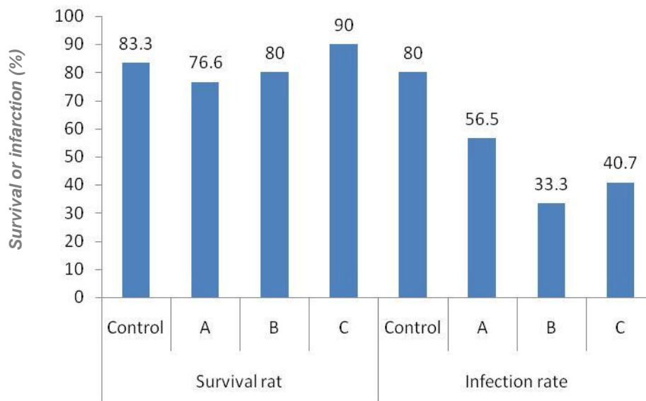
Figure 4. Effect of treatment with rice bran extract before [A], during [B] and after [C] infection with S. mansoni on survival and infection rate (%) of B. alexandrina .
