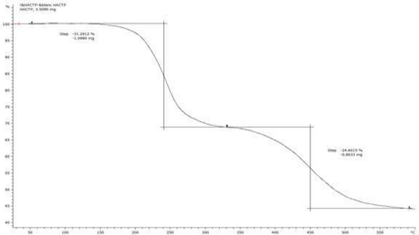
Figure 5. TGA curves of HACTP obtained in nitrogen atmosphere at heating rate of 10°C/min.
