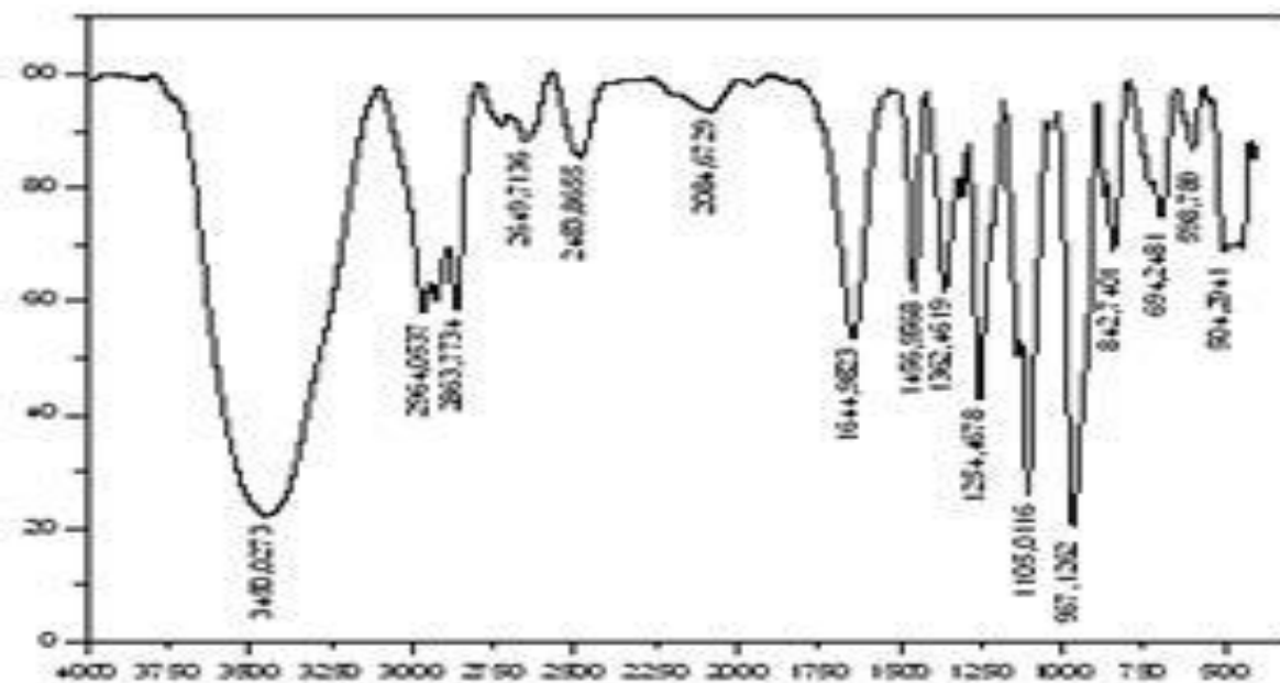
Figure 2. FTIR spectrum of HACTP induced by Maghnite- \text{H}^+ (0.25 M) at room temperature.
