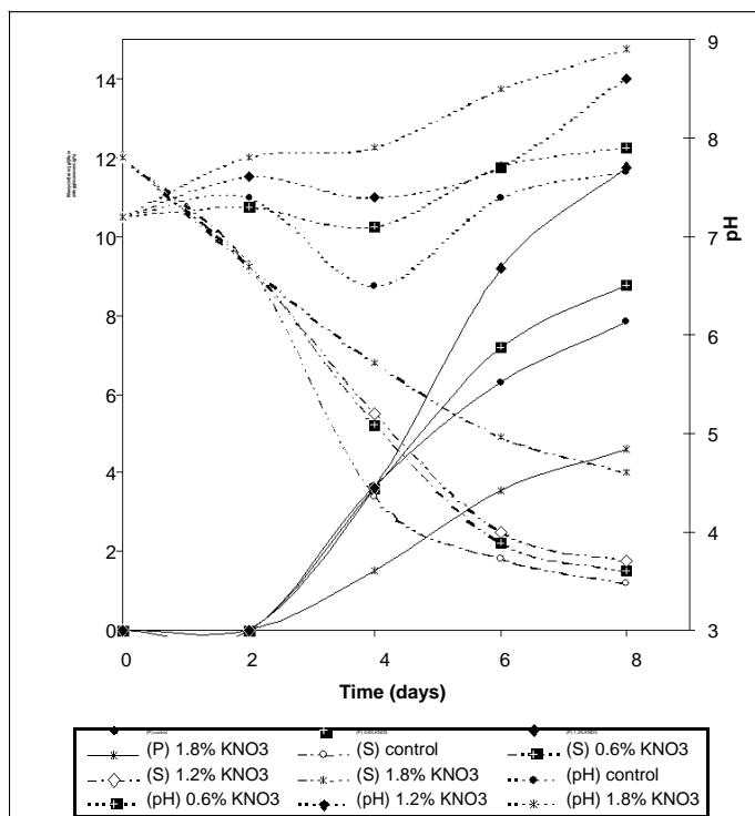
Figure 6. Effect of replacing (\text{NH}_4)_2\text{SO}_4 with \text{KNO}_3 in F2 medium on rifamycin B production (P), remaining glucose concentration (S) and pH by variant NCH.
