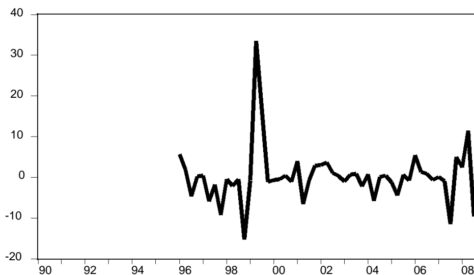
Figure 3. Brazil 1996 – 2008 sacrifice ratio.
