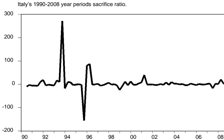
Figure 2. Italy's 1990-2008 year periods sacrifice ratio.
