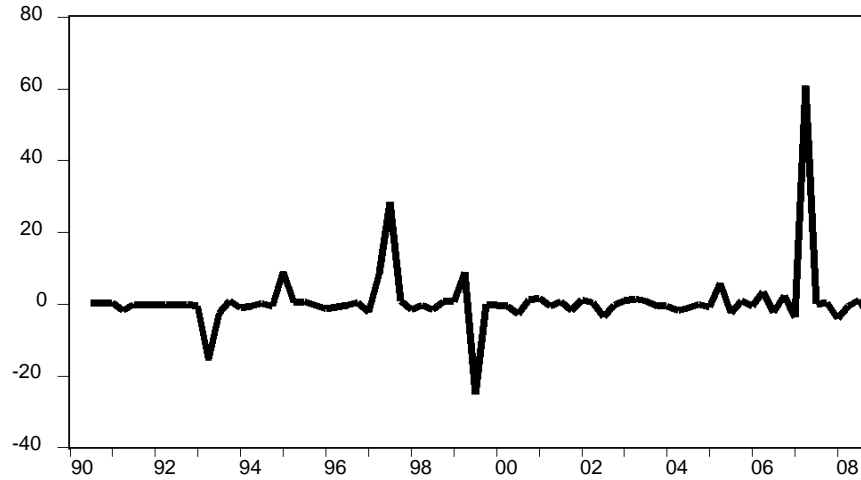
Figure 1. Turkey's 1990-2008 sacrifice ratio graph.
