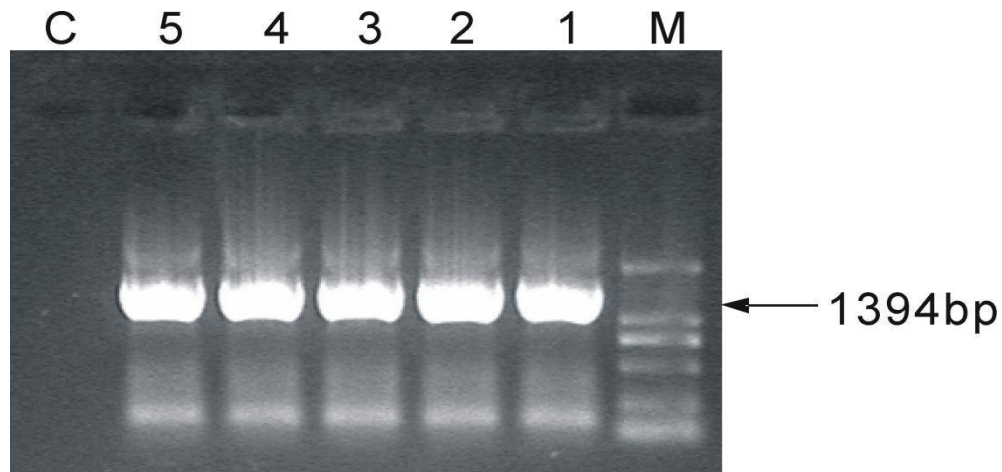
Figure 5. FRT-kan-FRT . Lane 1 shows the fragment synthesized with pKD13 plasmid as a template; Lane 2 and 3, fragments synthesized with the intermediary strain E. coli BW25113 phoA/FRT-kan-FRT genomic DNA as a template; lane 4 and 5, fragments synthesized with the intermediary strain E. coli BW25113 phoA/FRT-FRT/FRT-kan-FRT,phoA* genomic DNA as a template; Lane C, a negative control.
