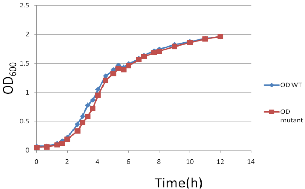
Figure 9. The mutant growth curve of the wild-type BW25113 and its mutant E. coli BW25113 phoA FRT-FRT/FRT-FRT phoA *( phoA gene at 97.1 - 97.2 min) realized after inoculation of a single colony of each in LB, incubated at 30°C for 16 h; 2.5 ml of these culture were diluted in 250 ml and incubate at 30°C and the OD600 was measured every 20 min. The data for the two strains were statistically analyzed by the correlation test.
