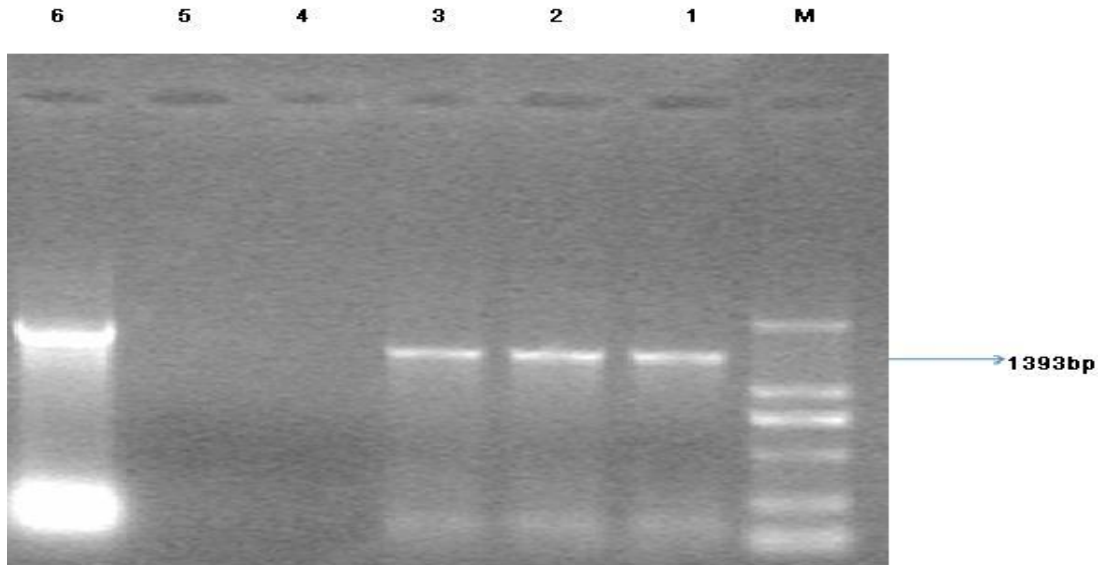
Figure 8. phoA gene expression using reverse transcriptase-PCR. Reverse-transcribed cDNA from the mutant E. coli BW25113 phoA FRT-FRT/FRT-FRT, phoA *( phoA gene at 97.1-97.2 min) total RNA was analyzed for the presence of a 1393-base pair (lanes 1, 2 and 3). The PCR fragment, a sequence from phoA gene was obtained with the primers PhoAex1 and PhoAex2. Two negatives controls were conducted (lanes 4, 5) without the total RNA as template and without the reverse transcriptase in the RT reaction, respectively. The lane 6 represented the phoA gene PCR product (1566 bp) using phoA 1 and phoA 2 primers using the E. coli BW25113 phoA FRT-FRT/FRT-FRT, phoA *( phoA gene at 97.1 - 97.2 min) genome as template.
