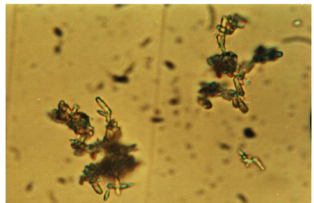
Figure 6. Extracts plants inhibited the aggregation phase of calcium oxalate crystallization
