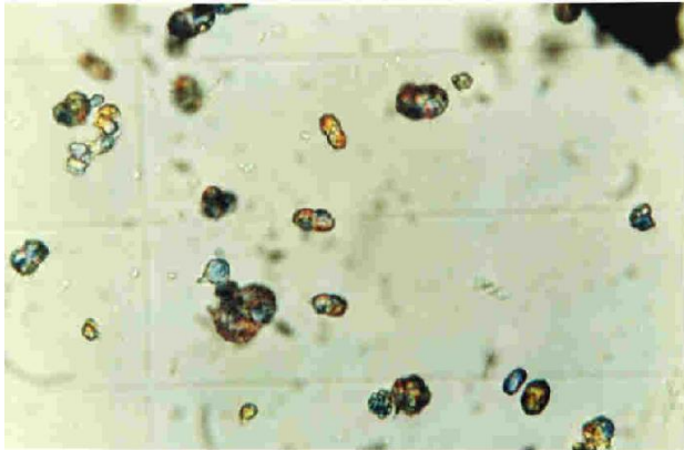
Figure 1. COM crystal nucleation in vitro
