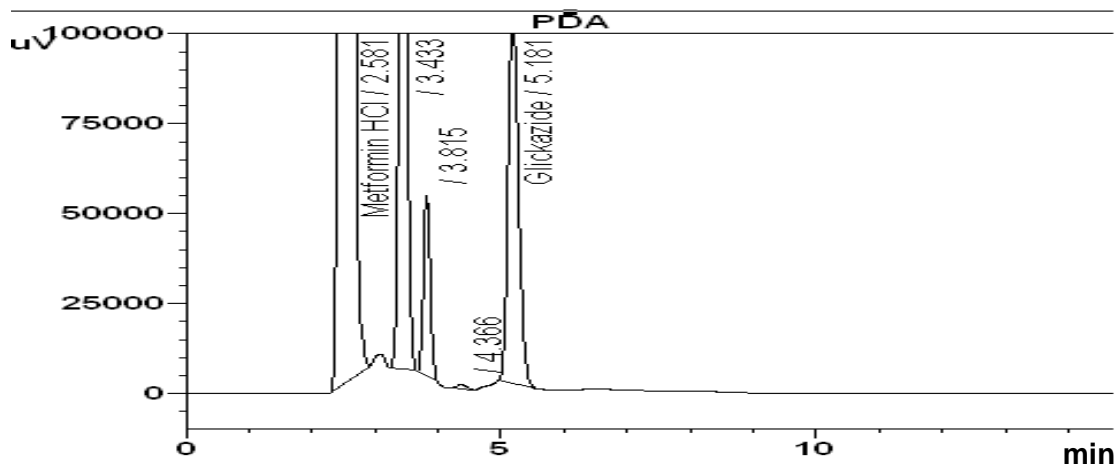
Figure 2d. Chromatograms of oxidative-degraded Metformin-hydrochloride and Gliclazide in tablet sample.
