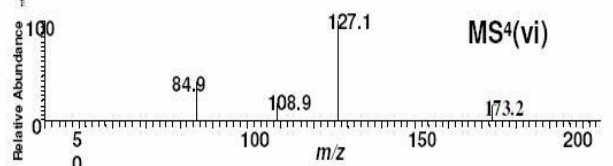
Figure 4. Represents a chromatogram of dicaffeoylquinic acid isomers: vi, vii, viii. MS 2 , MS 3 , MS 4 Spectra for 3,5 dicaffeoylquinic acid also indicated in the mass spectra.
