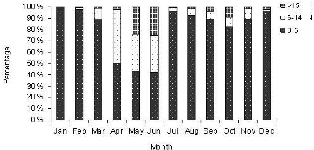
Figure 8. Percentage of M. leidy size (mm) frequency in different months in the southwestern Caspian Sea during 2001-2010.
