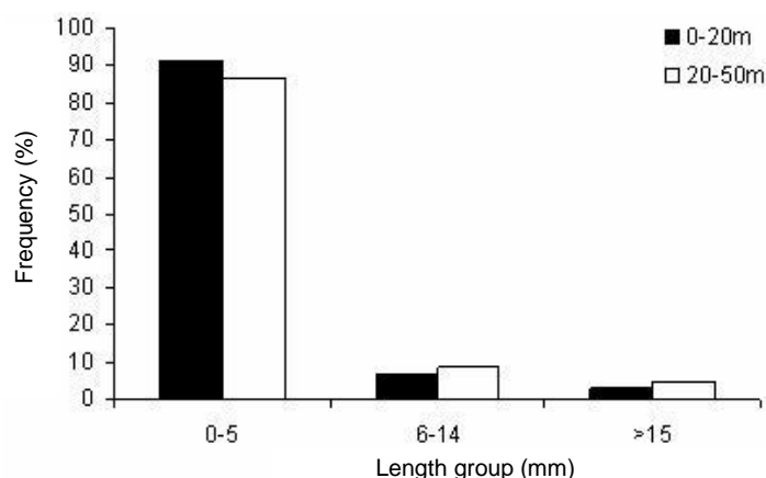
Figure 7. Comparison of size frequencies of the M. leidyi population from two layers in the southwestern Caspian Sea during 2001-2010.
