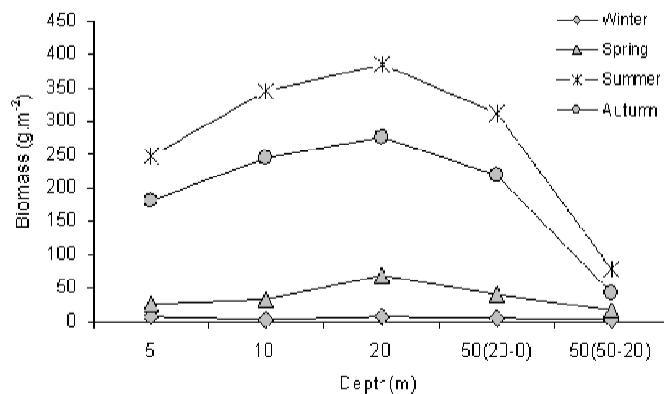
Figure 6. Temporal distribution of M. leidyi biomass in different seasons and depths in the southwestern Caspian Sea in 2004. Winter, spring, summer and autumn seasons were represented by February, May, July and November, respectively.
