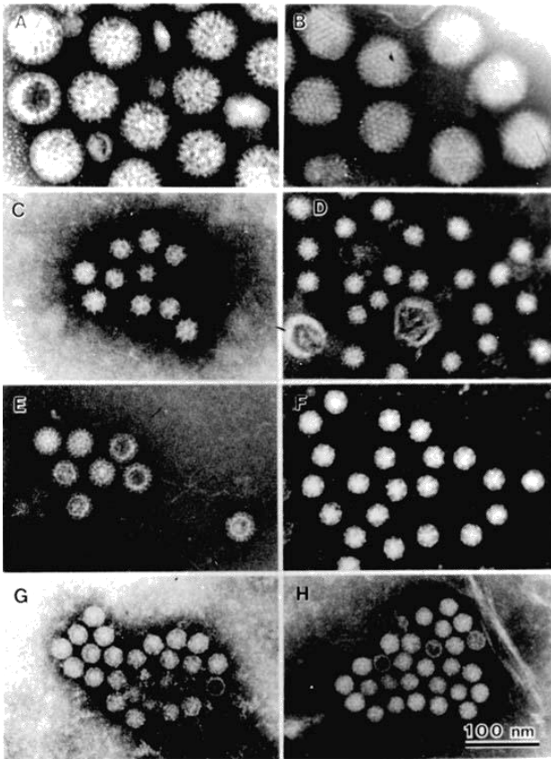
Figure 1. Representative Gastroenteritis Viruses. A, Human Rota virus; B, Human Adeno virus ; C, Sapovirus (Caliciviridae); D, Norovirus ( Caliciviridae); E, Otofuke Virus (Norovirus group); F, Human Astrovirus; G, ECHO Virus; H, Hepatitis A virus. Bar represents 100 nm.
