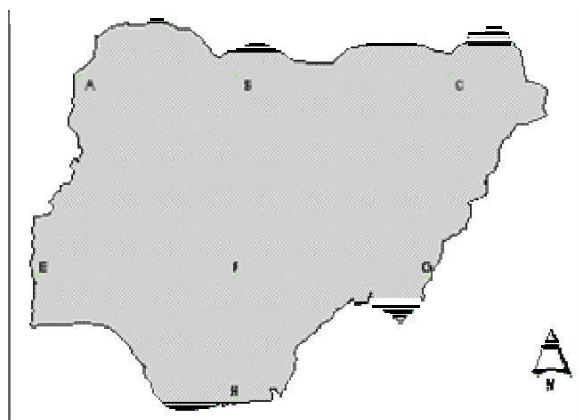
Figure 1. Map of Nigeria showing the points developed to run MAGICC-SCENGEN.
