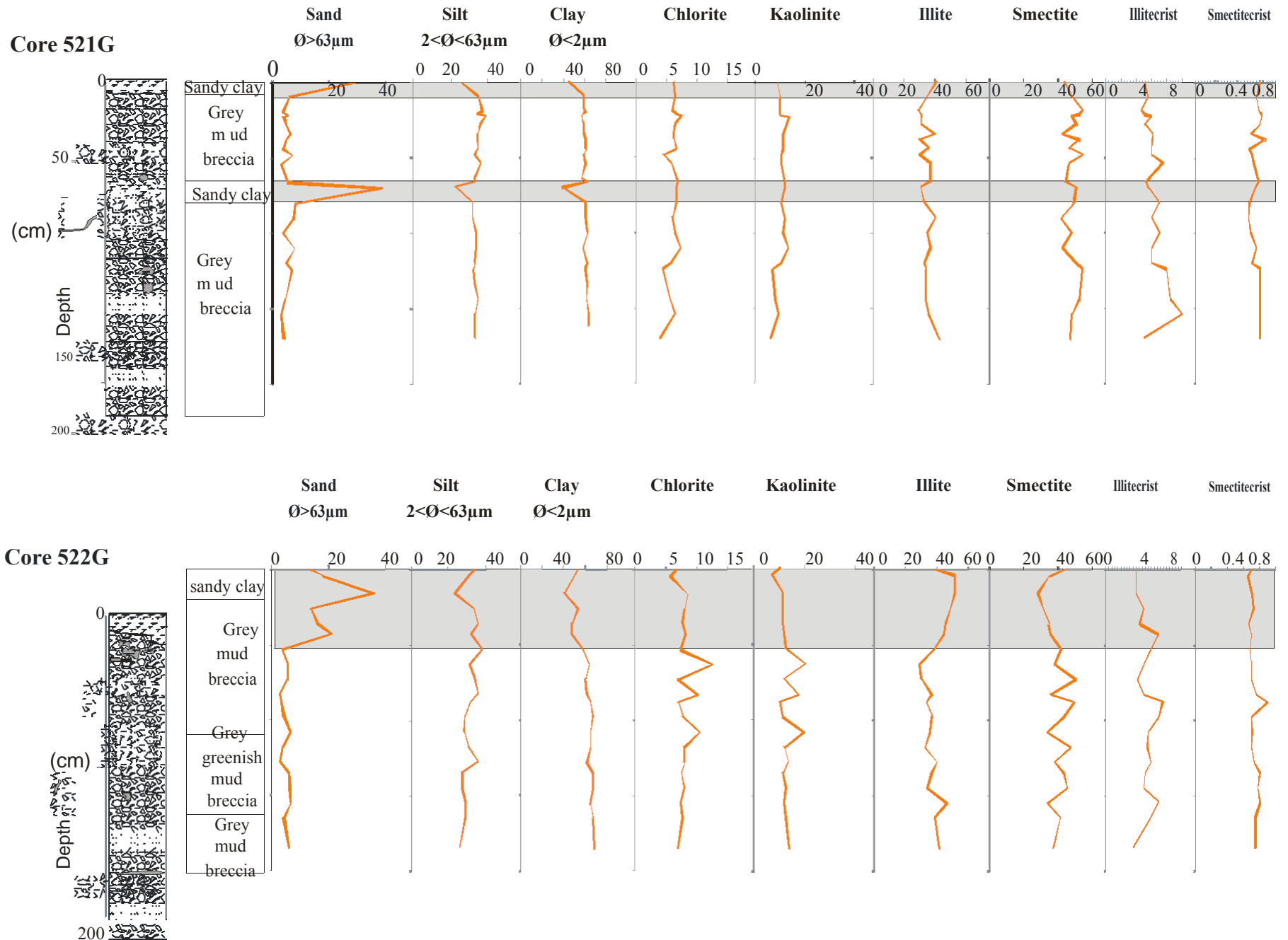
Figure 3. Main lithologic unit, granulometry and clay minerals at Ginsburg mud volcano.
