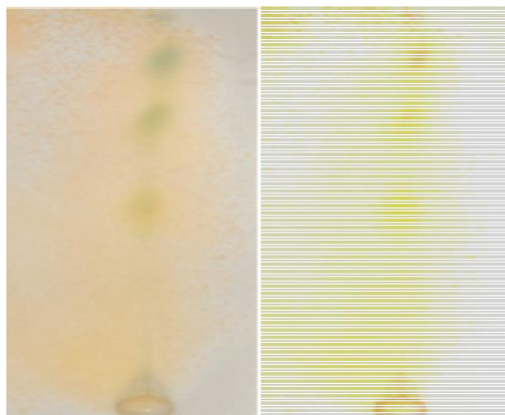
Figure 4. TLC profile, long uv (366 nm) derivatized, TLC profile of methanolic extract of Trichosanthes dioica , solvent system: toluene: ethyl acetate: diethylamine (7:2:1) spray reagent Dragendroff's.
