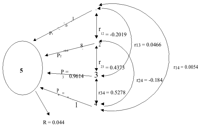
Figure 1. Nature of causal system of variables for the path-coefficient analysis in sorghum (1) Panicle length (2) Panicle count (3) Head weight (4) Grain mass (5) Grain yield (R) residual factors (r) correlation coefficient (p) unilateral path way. Double arrowed lines denote mutual association as measured by correlation coefficients, while single arrowed lines denote direct influence and measured by the path coefficient analysis.
