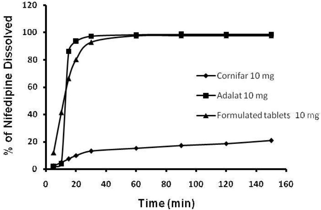
Figure 3. Dissolution profile of formulated tablets of nifedipine-HP-beta-cyclodextrin (10 mg) compared with commercial nifedipine products; Adalat® soft gelatin capsule (10 mg) and Cornifar® film coated tablets (10 mg).
