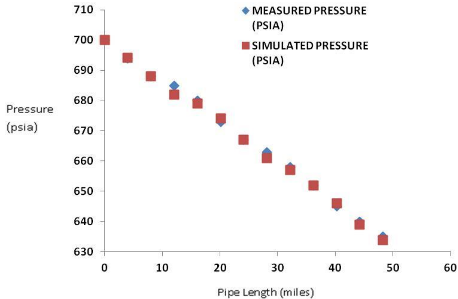
Figure 3. Plot of simulated and measured pressure vs. pipe length.
