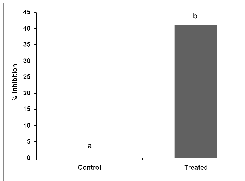
Figure 4. Growth inhibition (%) of Celosia argentea exposed to treated textile effluent. The values are the mean of four replicates \pm SE. ANOVA significant at p < 0.05 . Columns with different letters are significantly different.
