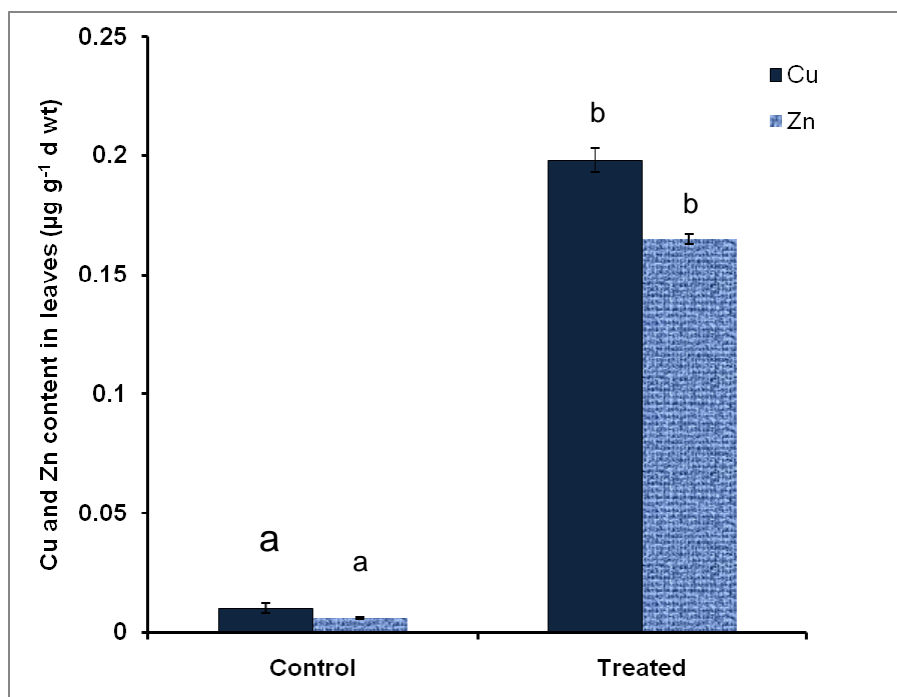
Figure 7. Copper and zinc content in leaves of Celosia argentea exposed to a treated textile effluent. The values are the mean of four replicates \pm SE. ANOVA significant at p < 0.05 . Columns with different letters are significantly different.
