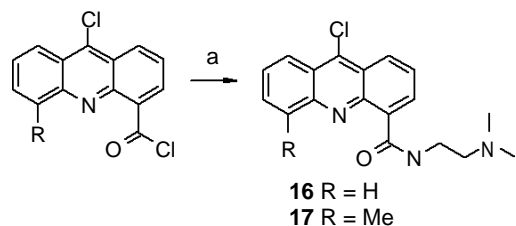
Scheme 5. a) 0°C, dichloromethane, N, N-dimethylethylene diamine, 64% overall.
