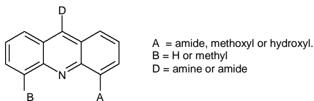
Figure 3. Acridine derivatives synthesized.
