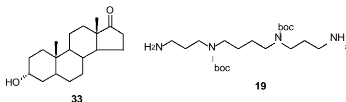
Figure 5. Androsterone and di-Boc spermine.
