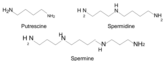
Figure 1. Naturally occurring polyamines.
