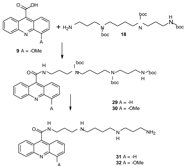
Scheme 9. a) Coupling agent (DCC, HOBt, or EDAC).
