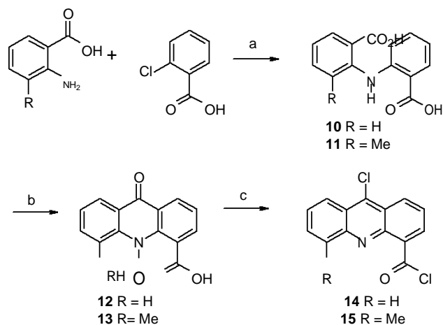
Scheme 4. a) DIPEA, DMF, Cu(OAc) 2 , 12 h, 120 °C, 75%. b) polyphosphoric acid, 120°C, 3 h, 70%. c) i) SOCl 2 , 80°C 1 h, 95% ii) N, N-dimethylethylene diamine, CH 2 Cl 2 , 0°C.
