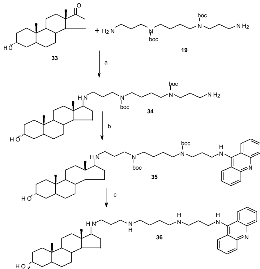
Scheme 11. a) BAP, dry, THF/MeOH, RT, 12 h, Acetic acid, 60%. b) 9-Phenoxyacridine, phenol, 120^\circ\text{C} , 70%. c) TFA, \text{CH}_2\text{Cl}_2 , 2 h, RT, 90%
