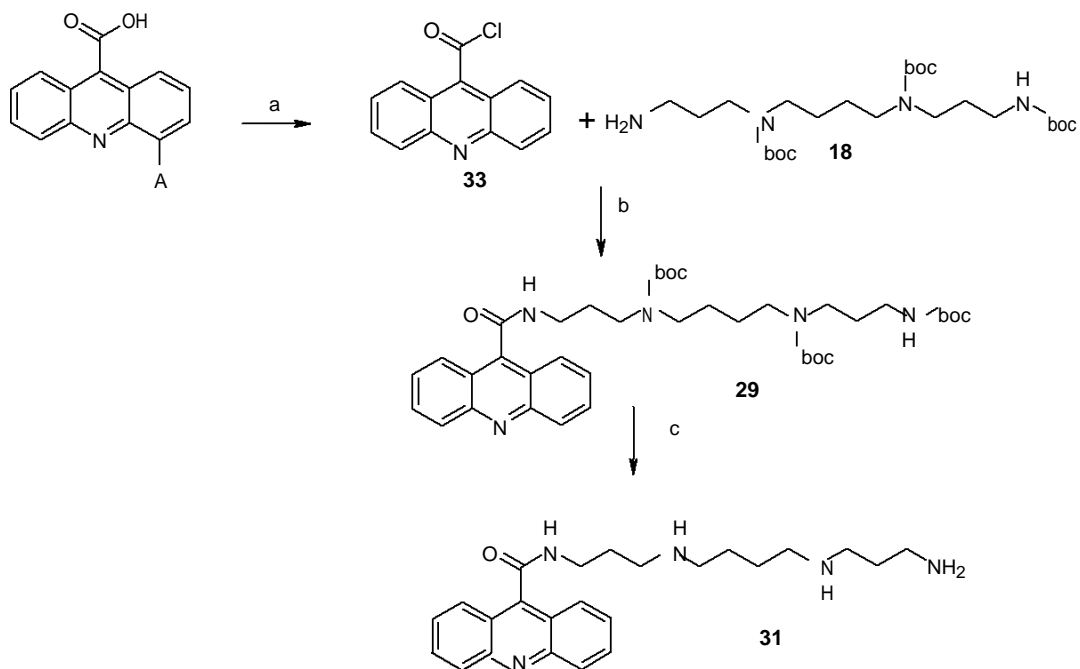
Scheme 10. a) \text{SOCl}_2 , 80^\circ\text{C} , 1 h, 95%. b) \text{CH}_2\text{Cl}_2 , DIPEA, rt, 2 h, 50%
