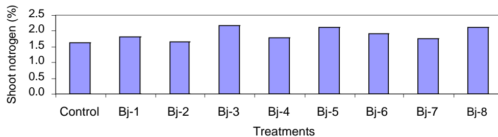
Figure 2. Effect of B. japonicum on nitrogen content in shoots of soybean cultivar PK 472.
