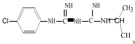
Figure 1. The Chemical Structure of Proguanil.
