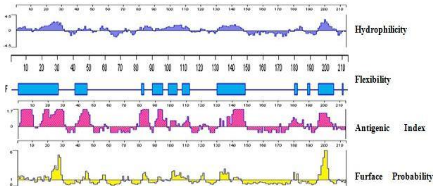
Figure 7. flexibility plot, hydrophilicity plot, surface probability plot and antigenicity index for structural protein VP1 of FMDV A/F72.
