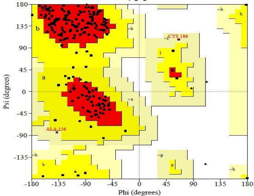
Figure 6. Ramachandran map of VP1 protein. The plot calculation on the three-dimensional (3D) model of VP1 protein was calculated with the PROCHECK program.
