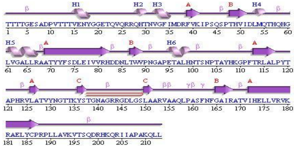
Figure 4. Secondary structure assignment of modeled VP1 protein.
