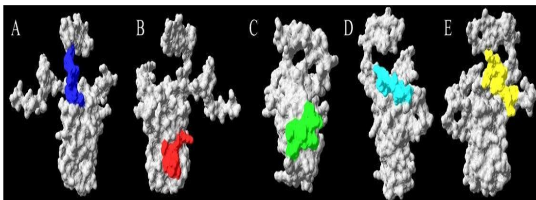
Figure 8. Putative exposed epitopes of VP1 protein mapped on molecular surfaces. Epitope regions of A (22-32aa), B (41-50aa), C (94-105), D (137-149aa) and E (196-205aa) are in blue, red, green, cyan and yellow.
