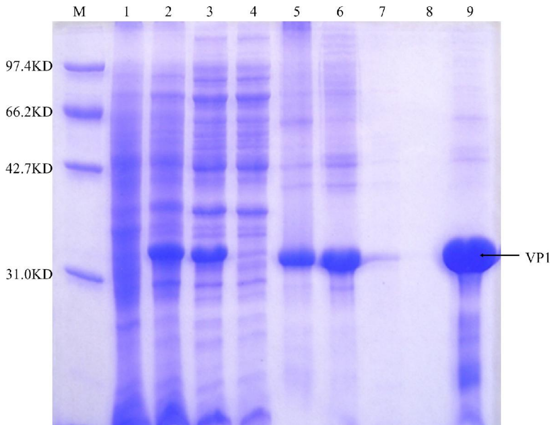
Figure 3. SDS- PAGE Results of VP1 protein. The results show that the structural protein VP1 after optimal expression has the size of 33 kDa, which is consistent with the expected size. 1. Uninduced control, 2. Inducing for 3 h, 3. Disintegrating liquid with ultrasonic, 4. Clarifying after disintegrating liquid with ultrasonic and centrifugation, 5. Purifying sample solution with Ni column, dissolved inclusion bodies, 6. Purifying flowing liquid with Ni column, 7. Purifying Ni- Denature-8.0 wash solution with Ni column, 8. Purifying Ni-Denature-6.0 wash solution with Ni column, 9. Purifying Ni-Denature-4.0 euate with Ni column.
