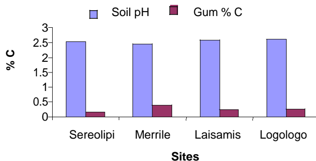
Figure 1. Comparison of Soil pH with % Carbon in Gum arabic in Sites.
