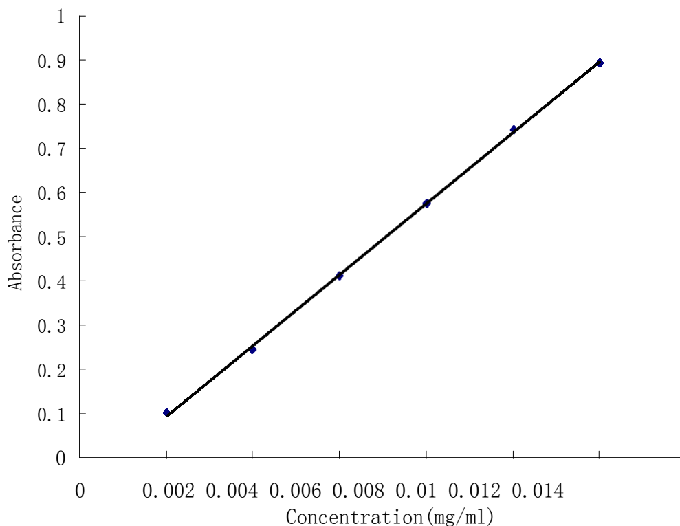
Figure 1. Standard curve of the measuring of the content of total flavone in Scutellaria baicalensis .
