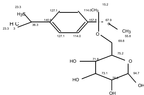
Figure 4. Structure of the active principle [6-(ethoxymethyl)-tetrahydro-2H-pyran-2, 3, 4, 5-tetraol compound with 1-isopropyl-4-methoxybenzyl].
