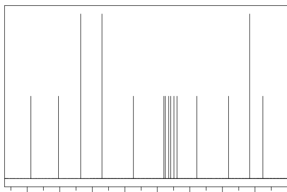
Figure 3. ^{13}\text{C} NMR spectroscopy of the active principle.
