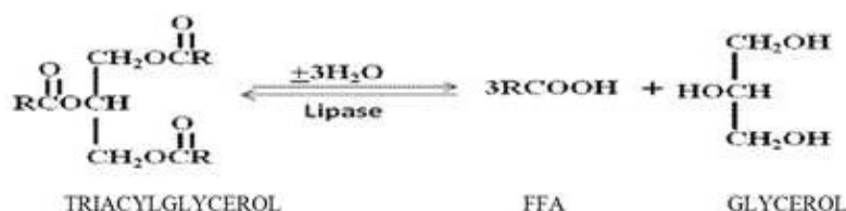
Figure 1. Origin of oil acidity (Patil et al., 2011).
