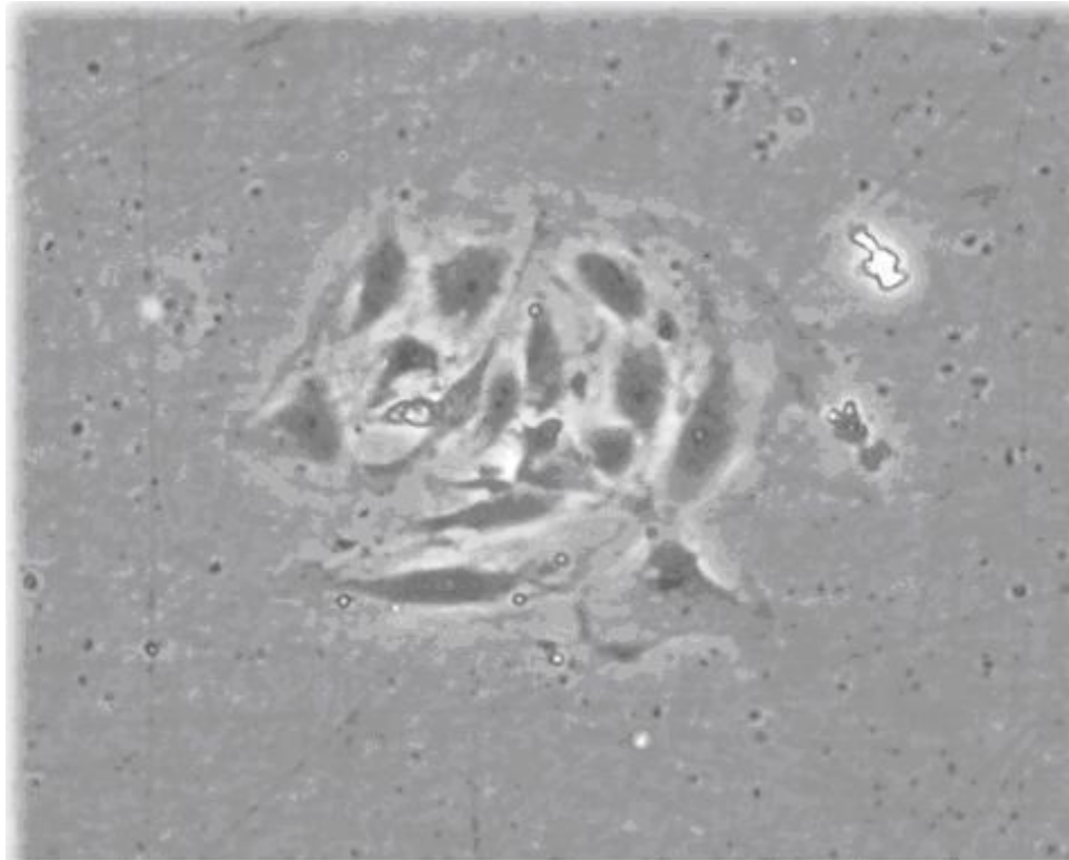
Picture 1. Small colony of DPSCs 24 h following inoculation. DPSCs are 12-18 \mu\text{m} in diameter. Phase contrast microscopy, direct magnification \times 200 .
