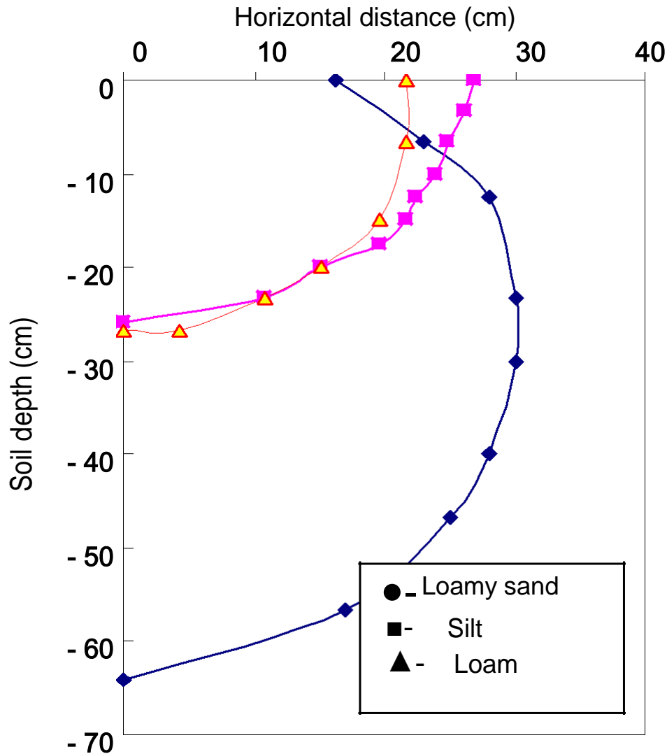
Figure 8. Predicted wetting front for overlap zone under different soil texture of drip irrigation.
