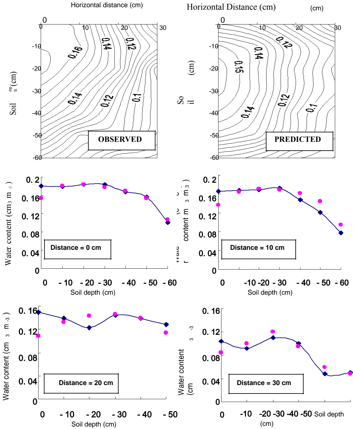
Figure 3. Measured and predicted water contents with irrigation volume 12 L.
