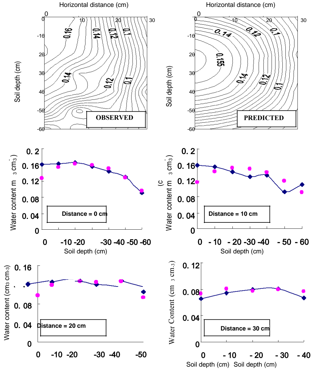
Figure 2. Measured and predicted water contents with irrigation water volume of 10 L.
