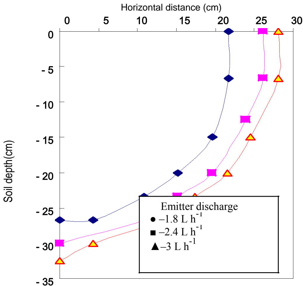
Figure 7. Predicted wetting front for intersection zone under different emitter discharge of drip irrigation.
