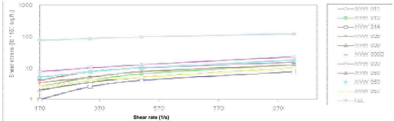
Figure 7. Rheological behaviour of unbeneftiated samples investigated at 22.5 g / 350 ml of clay concentration with imported bentonite (I.B.) as control at 22.5 g / 350 ml. NWY: Represent cardinal points where the samples were taken (N-North, W - West and Y is just to complement the name).
