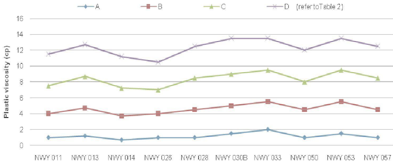
Figure 11. Effect of beneficiation and increase in clay concentrations on plastic viscosity. NWY: Represent cardinal points where the samples were taken (N-North, W - West and Y is just to complement the name). I.B: Imported Bentonite – represent commonly used drilling fluid by the industry. A, B, C, and D: Different composition of mud preparation for laboratory experiment (Table 2).
