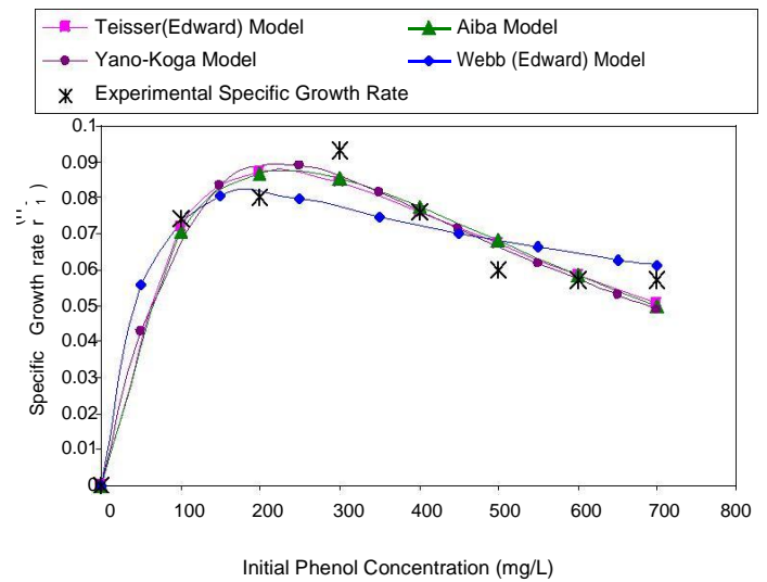
Figure 5. Experimental and predicted specific growth rate of the culture due to Teisser (Edward), Webb (Edward), Yano-Koga and Aiba model.
