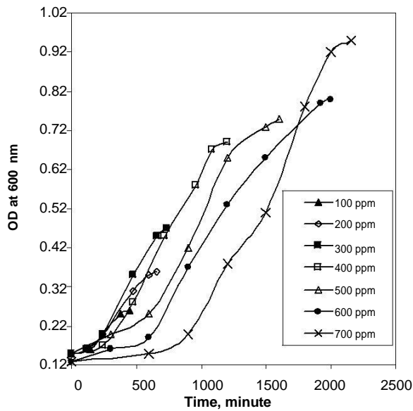
Figure 2. Microbial growth profile with time.
